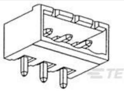
TE Part #796638-3 3POS 5.08MM CE R/A HDR,TRM BLK
