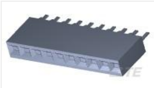
TE Part #534237-8 10 MOD II VRT SR CE 100/115
