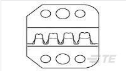
TE Part #90548-2 PROCRIMPER DIE ASSY UNIV MNL
