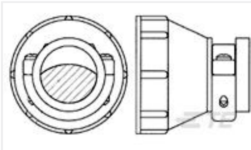
TE Part #182661-1 CPC Cable Clamp Kit, Size 17, Large, UV
