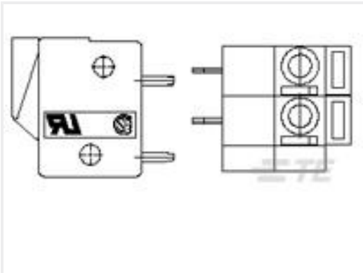
TE Part #1776261-4 4P Spring TB, 90deg, VT,5mm, Green
