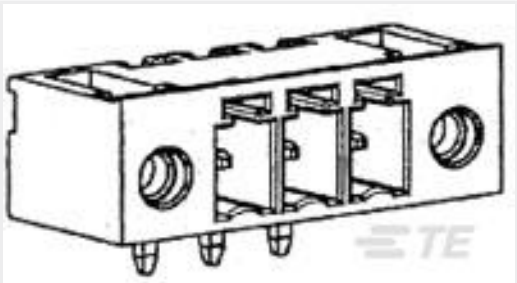
TE Part #284541-4 4 POS TERMI-BLOK 900 SF 3,81 m
