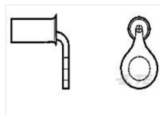
TE Part #321867-1 TERM,SOLIS R 1/0 5/16 90DEG
