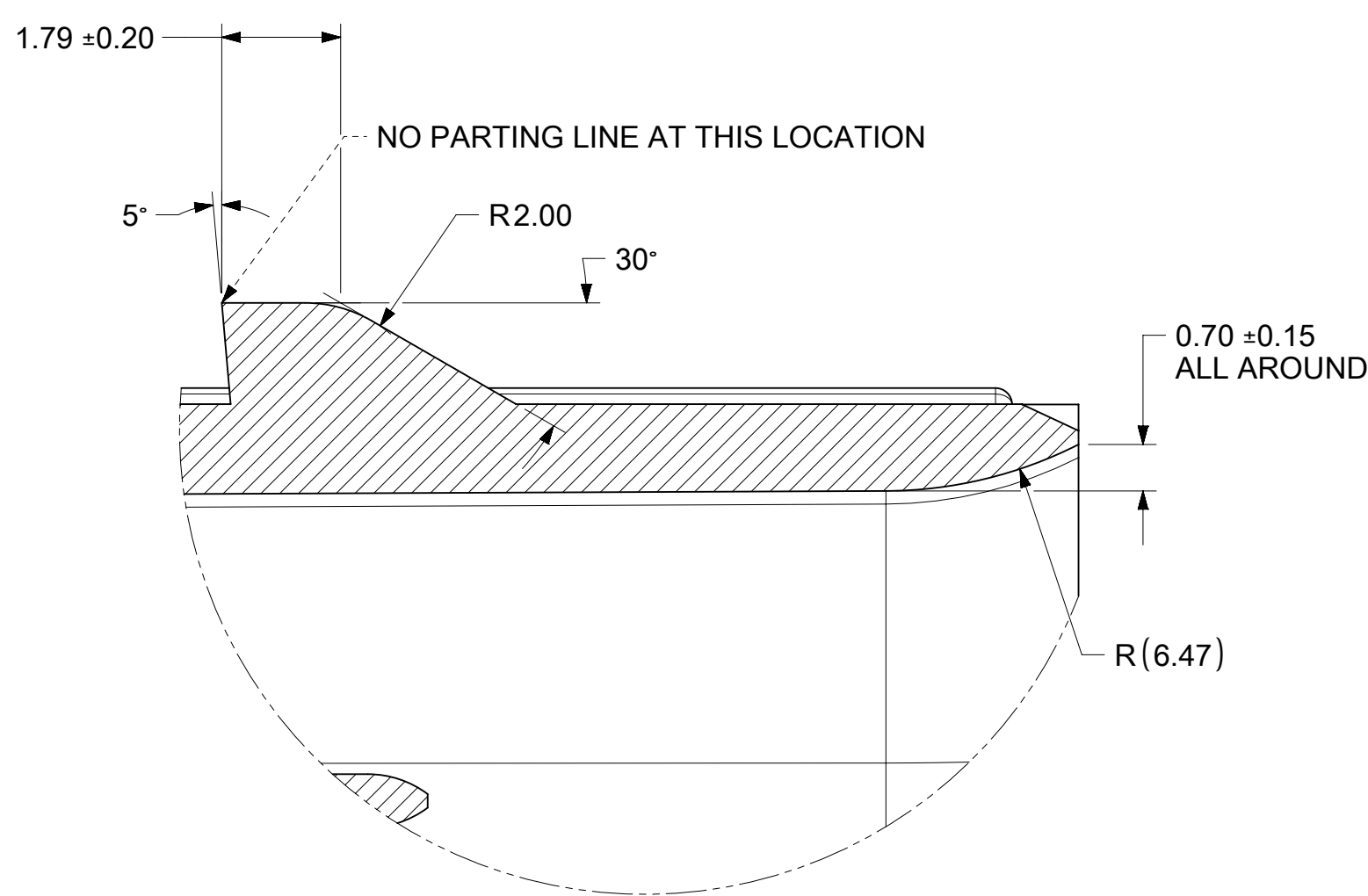
DETAIL 3 SCALE 10:1
