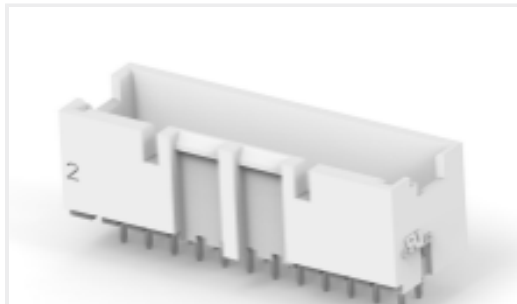
TE Part #2-2324245-4 ASSY,HDR,VERT,GWT,BOSSD,DUAL ROW, EP2.5
