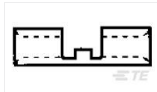
TE Part #323698 SPLICE,SOLIS BUTT HT 12-10
