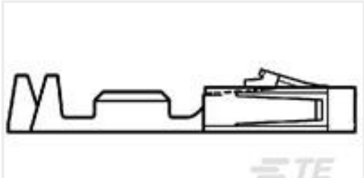
TE Part #1-104479-1 SHORT POINT RECP CONT LP
