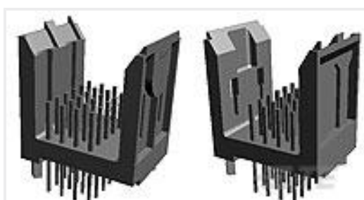
TE Part #1-179554-3 Receptacle and Tab Housing: 5.08 mm Pitch, 250-600V
