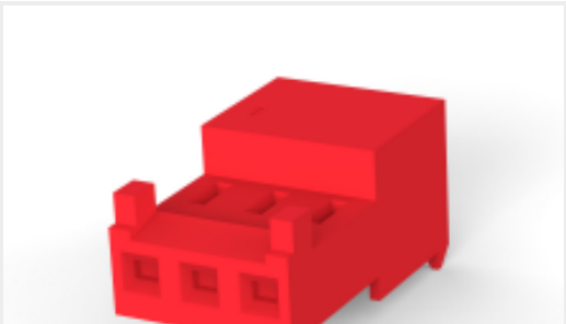
TE Part #3-643813-8 Nylon Tin Plated Receptacle: 2.54 mm, with Mating Alignment, MTA 100
