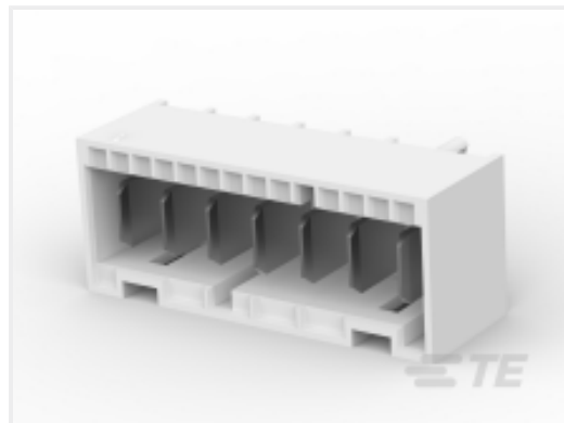
TE Part # 1971845-7 7P, RAST 5 Tab Header, THV
