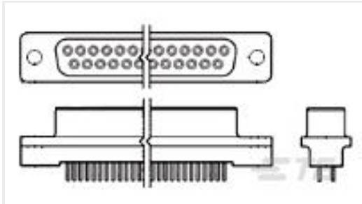
TE Part #5745079-4 HD-20 RCPT 37P VERT FFSCRLK
