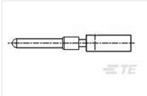
TE Part #5-1437720-5 T01-CRIMP-P05=TRIAD
