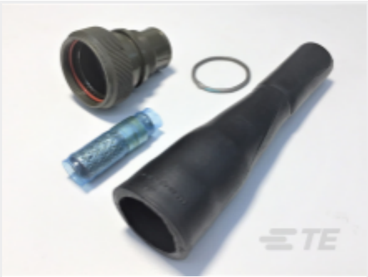
TE Part #104739-000 5428-12-441116
