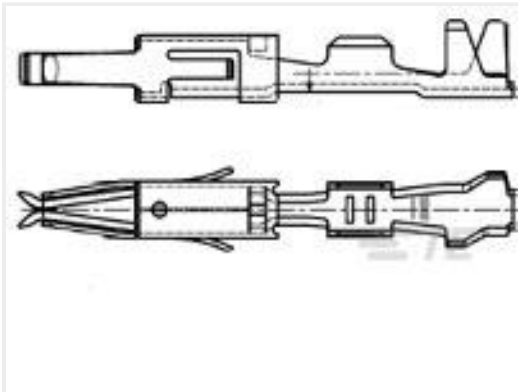
TE Part #1241844-2 MT2 A REC 1.6 Contact SRC Sn
