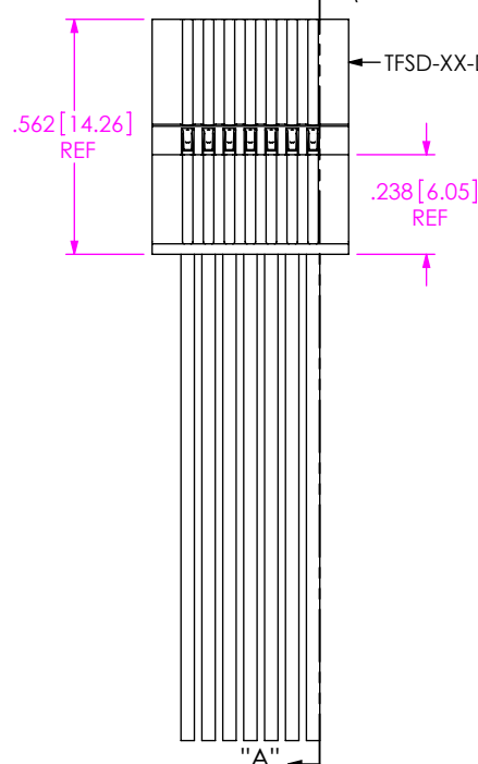
FIG 1 -S: SINGLE END (TFSDX-07-28-XX-XX-XX-S SHOWN)
