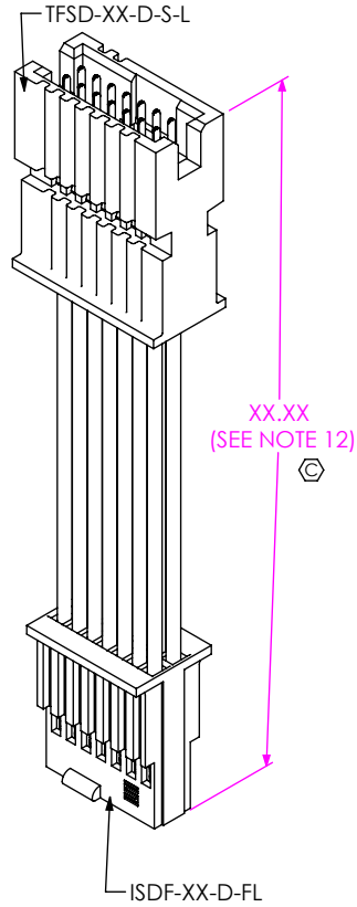
FIG 6 -TF: TRANSFER END WITH FRICTION LOCK (TFSDX-07-28-XX-XX.XX-TF-NUS SHOWN) (DIFFERENT AS SHOWN, OTHERWISE SAME AS FIG 1)
