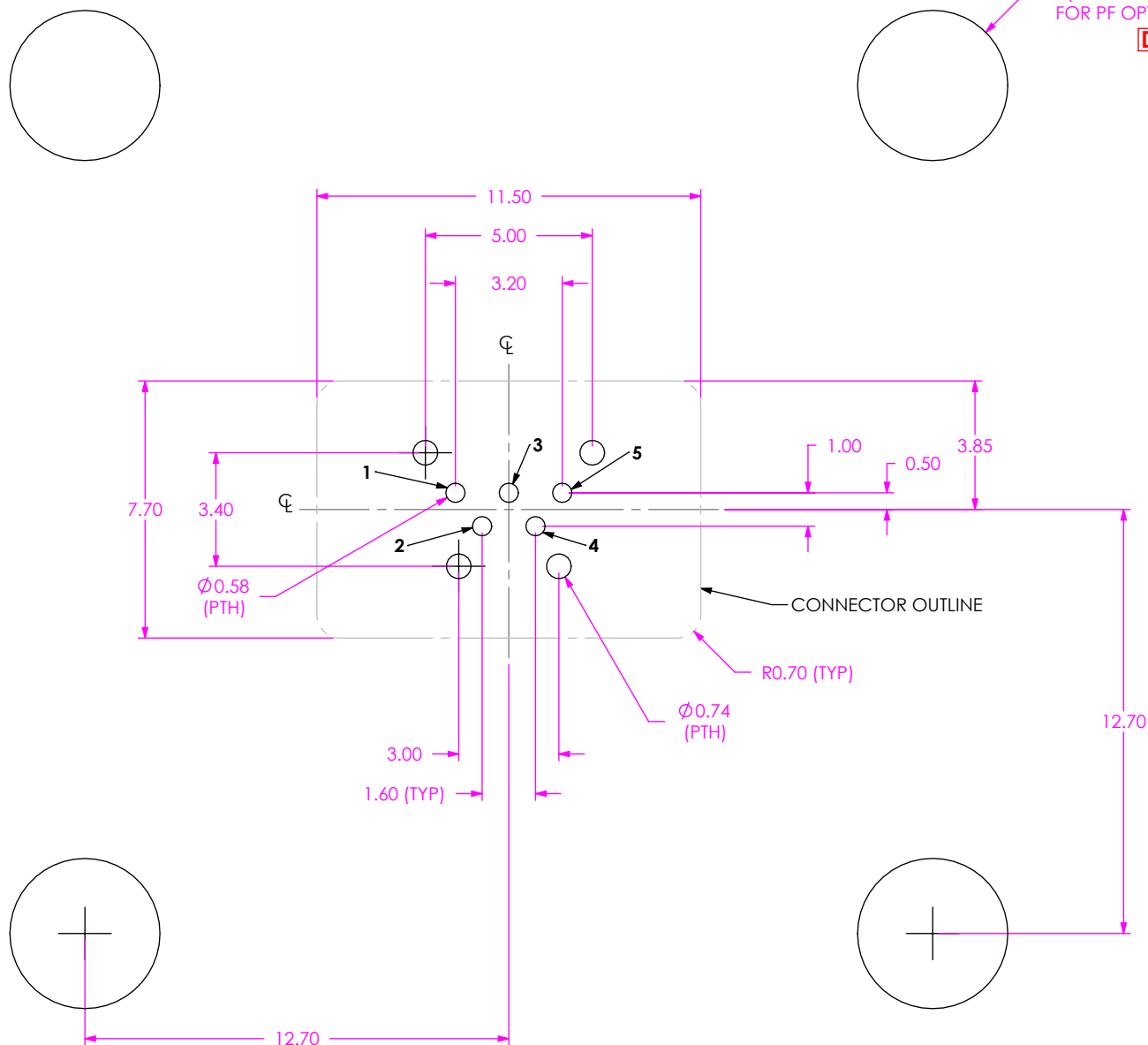
FIG 1 (MUSBS-05-S-B-TH-XX-TR SHOWN)
