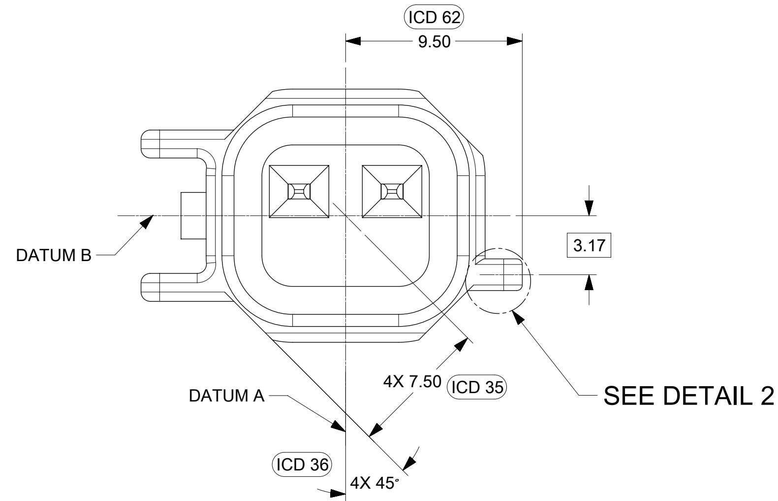
OPTION B
