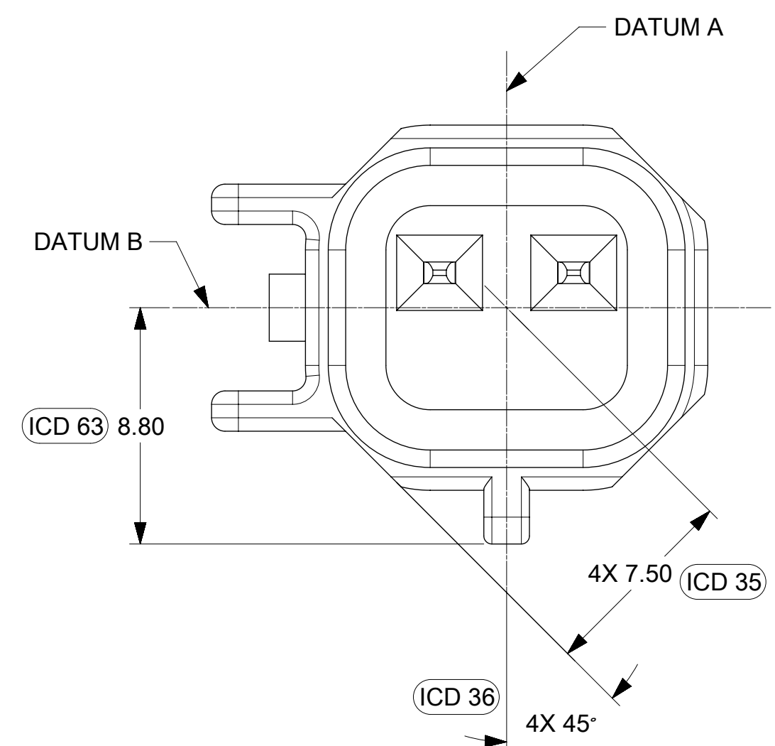
OPTION H
