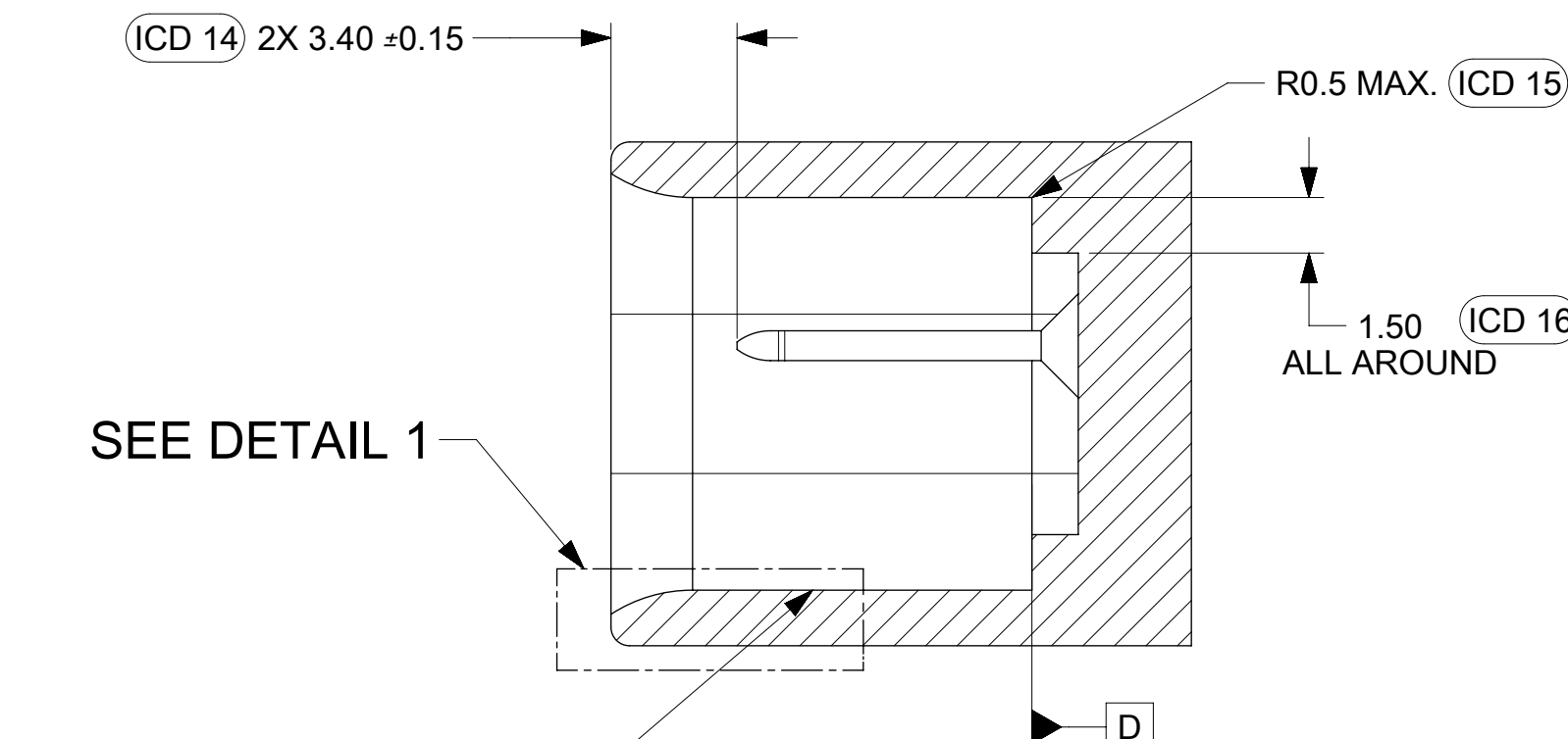
SECTION Y-Y
