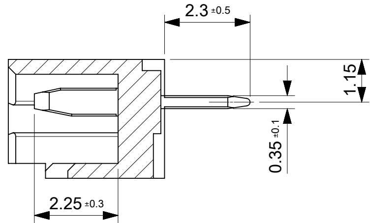
SECTION X-X
