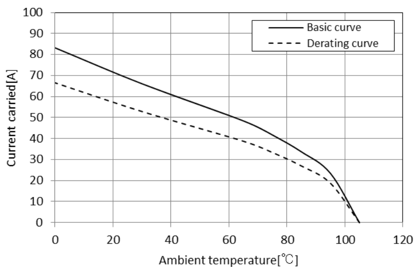
Derating curve
