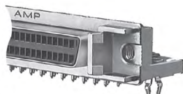
Right Angle Receptacle—Rails, Latchblocks, Boardlocks
