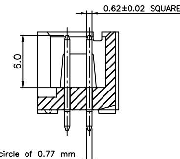
SECTION A-A WITHOUT CAP
