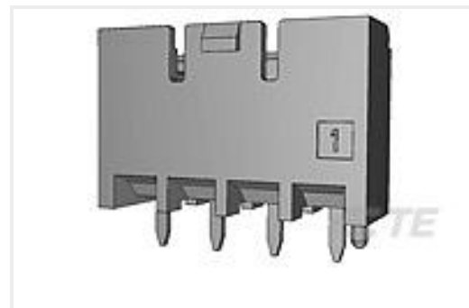
TE Part #1376384-1 5mm B-T-W Conn. 4P HDR ASSEMBL
