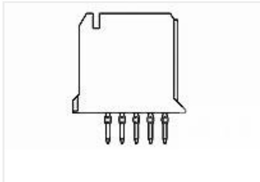
TE Part # 5223652-4 2MM FB,5RV,REC,ASY,120,PF,4.25
