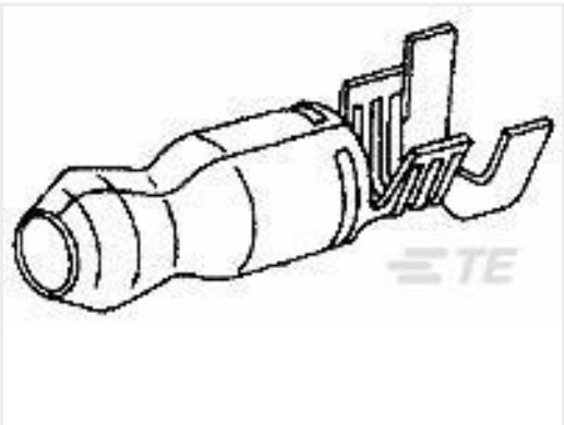
TE Part #505038-1 SHUR PLUG 180 CRIMP TAB 20-16 AWG BR
