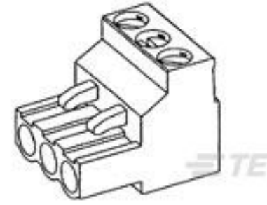
TE Part #796634-3 3 POS 5.08MM R/A PLUG, TRM BLK
