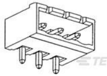
TE Part #796638-3 3POS 5.08MM CE R/A HDR, TRM BLK
