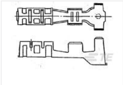
TE Part #175135-1 CONTACT 22-18 AWG 0.30 X 17.0 PTKLF-5
