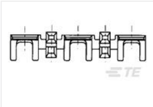
TE Part #353256-1 110 HSG. PL EX REC. 7.6mm 3P NAT
