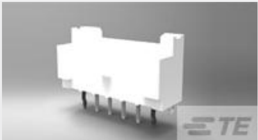
TE Part #2132415-8 EP2.5 Shrouded HDR ASSY 8P VERT w /o boss
