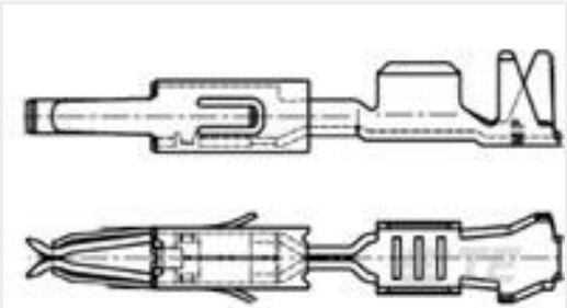
TE Part #1241860-2 MT3 REC 1.6 Contact SRC Sn
