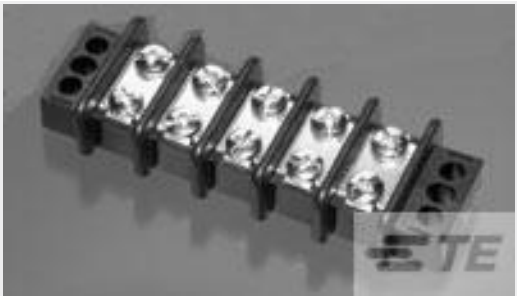
TE Part #1546310-4 4P .563" DR BARRIER STRIP
