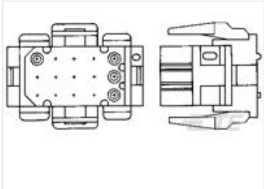
TE Part #1-640525-0 24P MR II PLUG HSG V0
