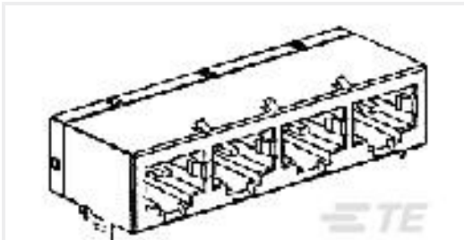
TE Part #5558524-1 MJ,1X4,R/A,8P,PNL GND,CAT5 NT
