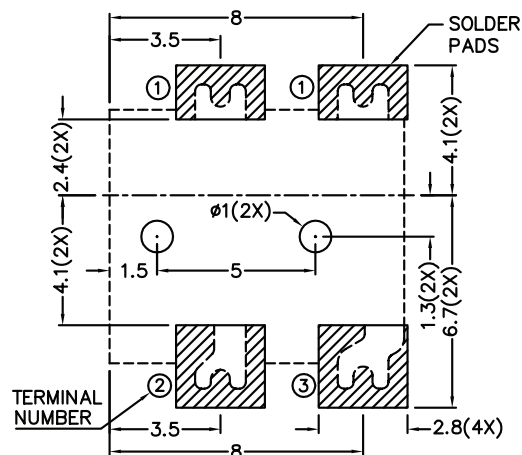
RECOMMENDED PCB LAYOUT TOLERANCE: \pm 0.05 (TOP VIEW)
