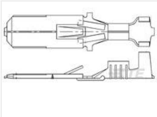
TE Part #170151-2 FF 250 TAB 18-14AWG PTBR
