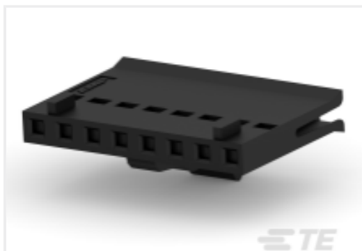
TE Part # 487526-7 008 HOUSING FFC RCPT 100CL SR
