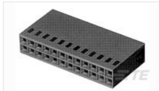
TE Part # 1-86177-1 40 MODIV HSG COMP DR .100CL
