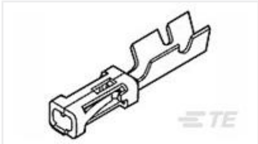
TE Part #102917-5 MOD IV RECP PLTD 15 SEL
