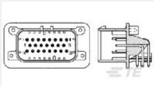
TE Part #776087-4 23POS,PIN DIA 1.3,HDR ASSY,90DEG, COD 4
