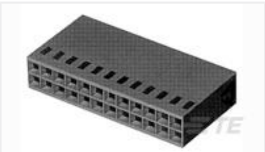
TE Part #87456-9 14 MODIV HSG COMP DR .100CL
