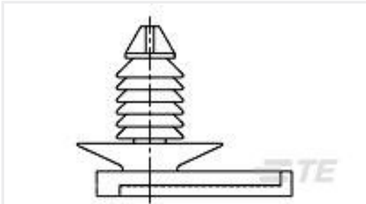
TE Part #368373-1 CLIP FOR EJ MK-II (TREE TYPE)
