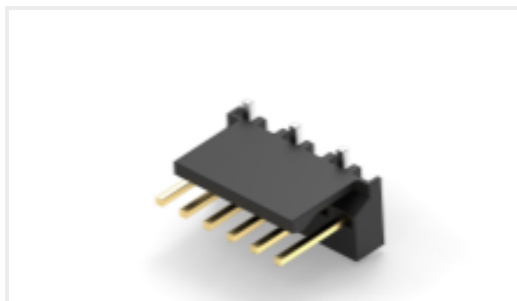
TE Part #3-647166-5 PCB Header: Nylon, Vertical, Surface Mount, MTA 100
