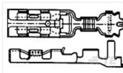
TE Part #353250-2 110 PL EX REC. 20-16AWG PTPHBZ
