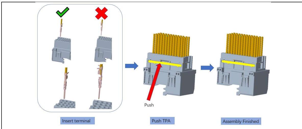
Figure 3.1.4 Terminal and TPA Assembly
