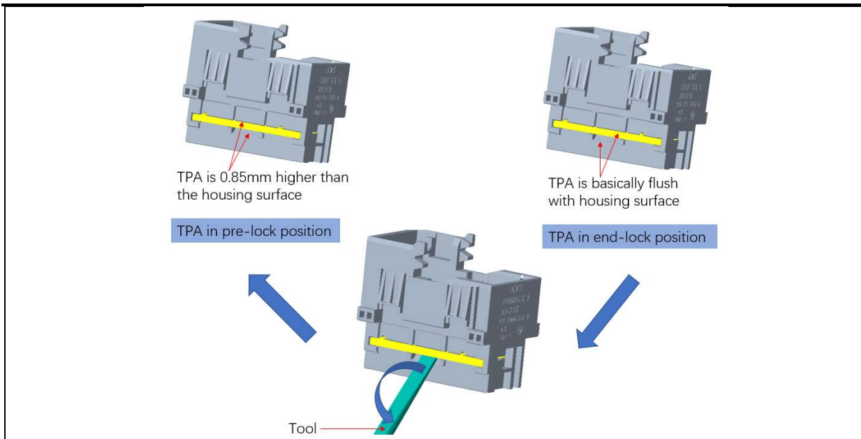
Figure 3.1.3 Check the Position of TPA
