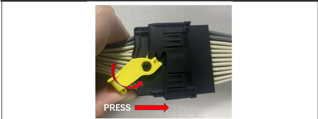
Figure 3.3.2 Preassembly Plug into Receptacle
