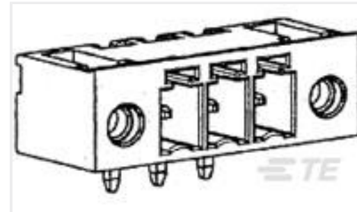
TE Part #284541-6 6 POS TERMI-BLOK 900 SF 3,81 m
