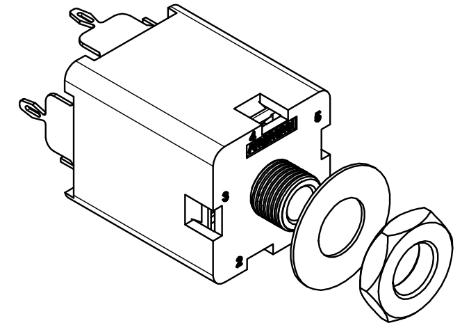
3D VIEW ( 2:1 )
