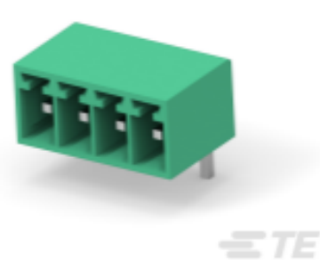
TE Part #2350514-4 4POS TB HDR 90 DEG, PITCH 3.5 & TL 3.5mm
