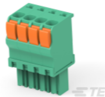
TE Part # 1986692-4 STR PLUG SPRING TYPE RH 4P, 3.50 mm
