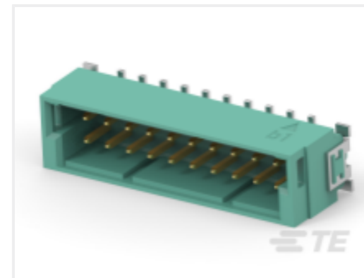
TE Part #464688-E DRCQ 2,54 20 M * SMD * 137 E012 167 GU-H
