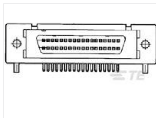
TE Part #5174225-1 AMPLIMITE 050-2B HOR 20P M2.5
