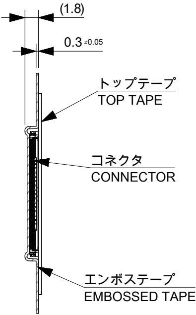
SECTION Y-Y
