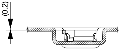
SECTION X-X
